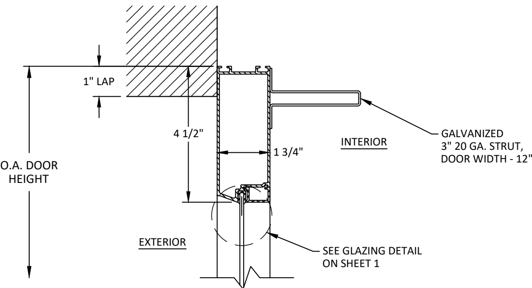
A 4 VERTICAL SECTION UPPER SECTION DETAIL
