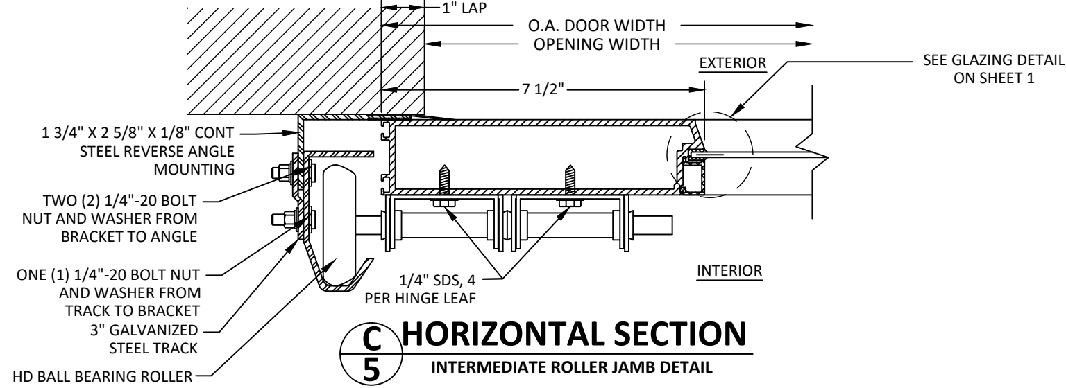
A HORIZONTAL SECTION 5 UPPER ROLLER JAMB DETAIL
