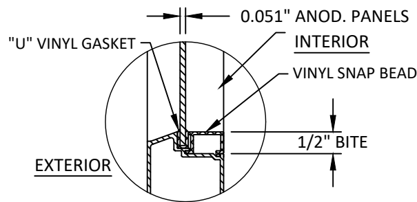
GLAZING DETAIL 2
