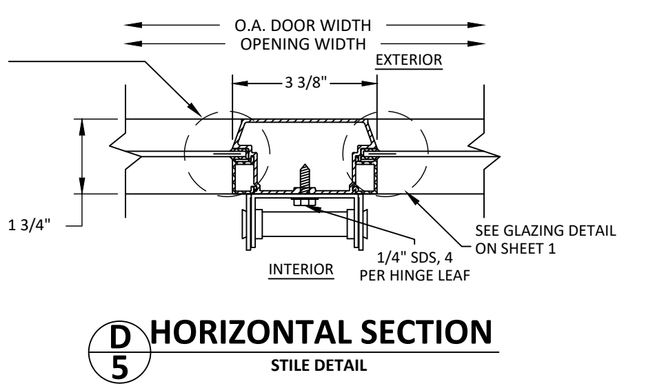
B HORIZONTAL SECTION 5 STILE DETAIL
