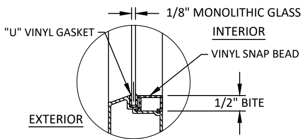
GLAZING DETAIL 1
