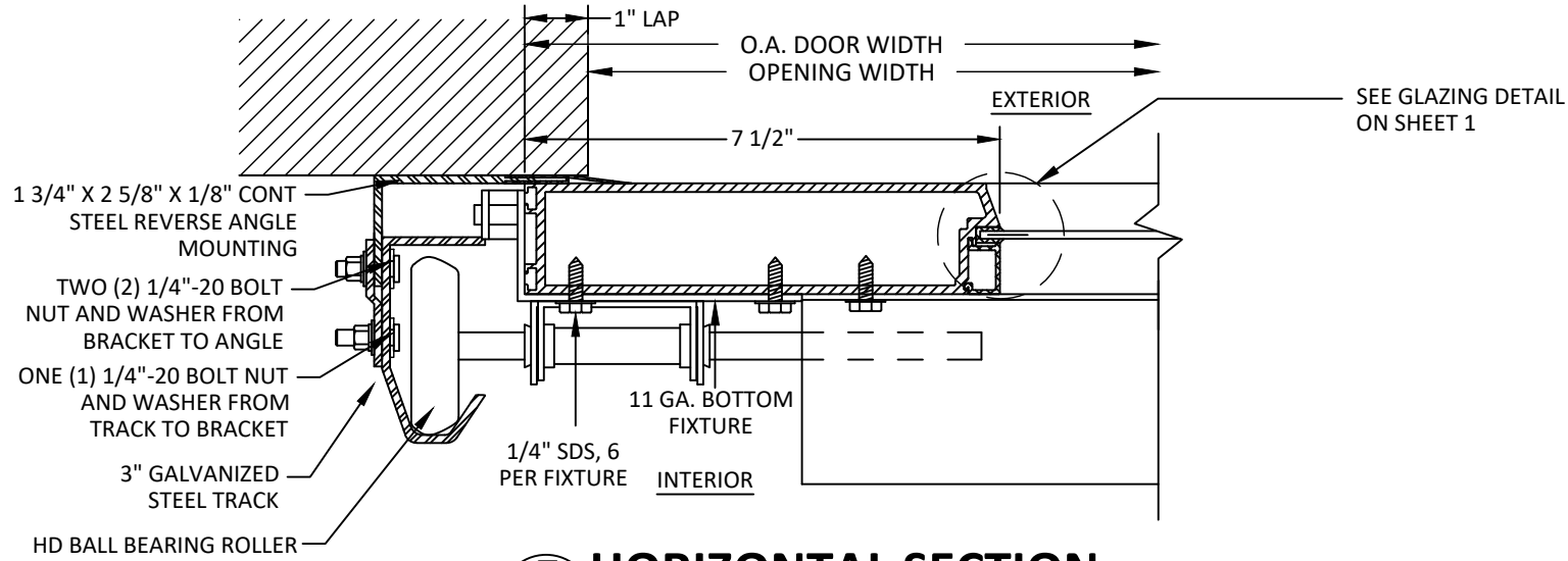
E HORIZONTAL SECTION 5 LOWER ROLLER JAMB DETAIL
