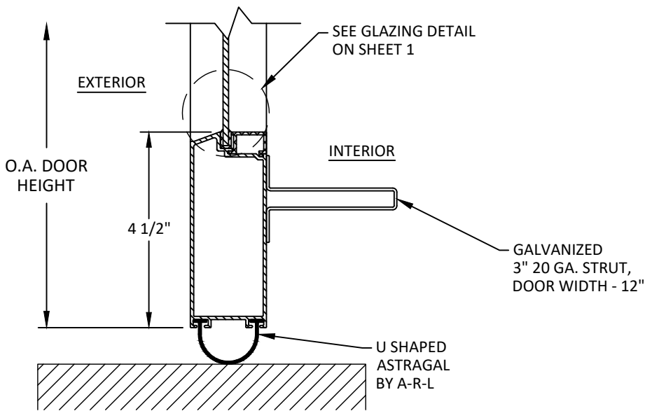
C 4 VERTICAL SECTION LOWER SECTION DETAIL
